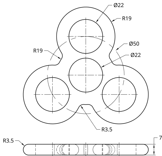
FIDGET SPINNER UNITS - mm MATERIAL - ABS
